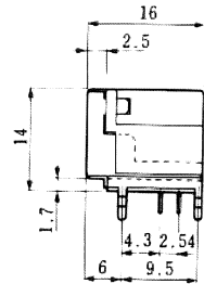
Board mounting dimensional drawing (connector side)
