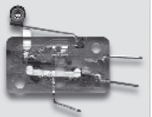
S840 r 20 Roller lever and flat tabs 6.3 x 0.8
