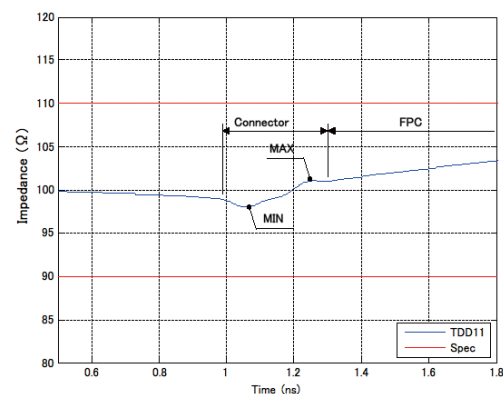
FH53 differential impedance 130ps rise time (20–80%)
