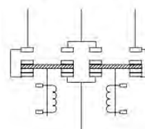
2 Pole - Double Throw
