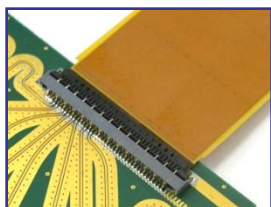
FH55 Series 0.5mm Pitch, High Speed Transmission
