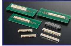
FX10 Series 0.5mm Pitch, 4-13mm Height, Floating structure High Speed Transmission
