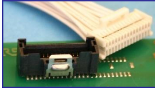
DF50 Series 1mm Pitch, Double-row Positive Lock
