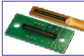
DF40 Series 0.4mm Pitch, 1.54.0mm Height
