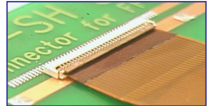
FH19C/FH19SC Series 0.5mm Pitch, 0.9mm Height
