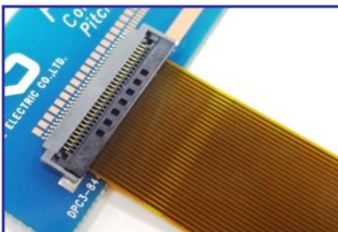
FH52E Series 0.5mm Pitch, 2mm Height
