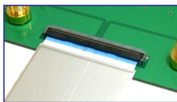
FH41 Series 0.5mm Pitch, Supports Shielded FFC
