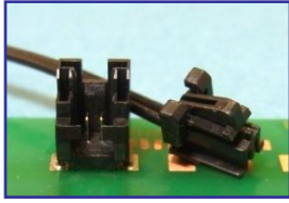
DF50A Series 1mm Pitch, Single-row Positive Lock
